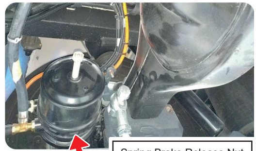
Spring Brake Release Nut
